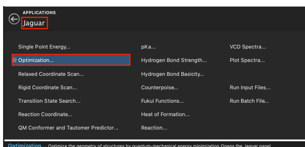
Figure 3-4. Opening the Jaguar Optimization panel.
