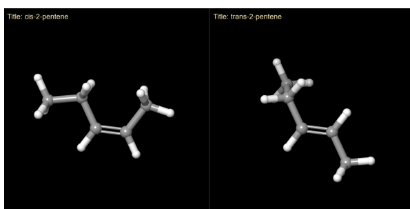
Figure 5-9. Viewing 2-pentene isomers.
