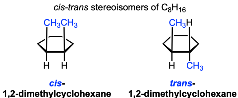
Figure 2-2. Cis-Trans isomers of C_8H_{16}
