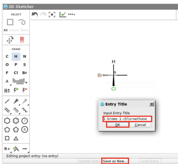
Figure 3-2. Drawing 1-bromo-1-chloroethane.
