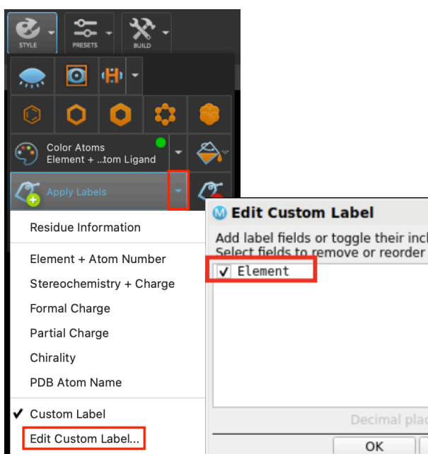
Figure 3-11. Labeling atoms.
