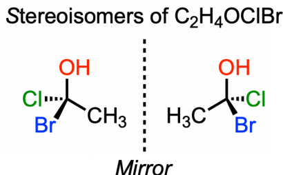
Figure 2-4. Stereoisomers of C_2H_4OCIBr
